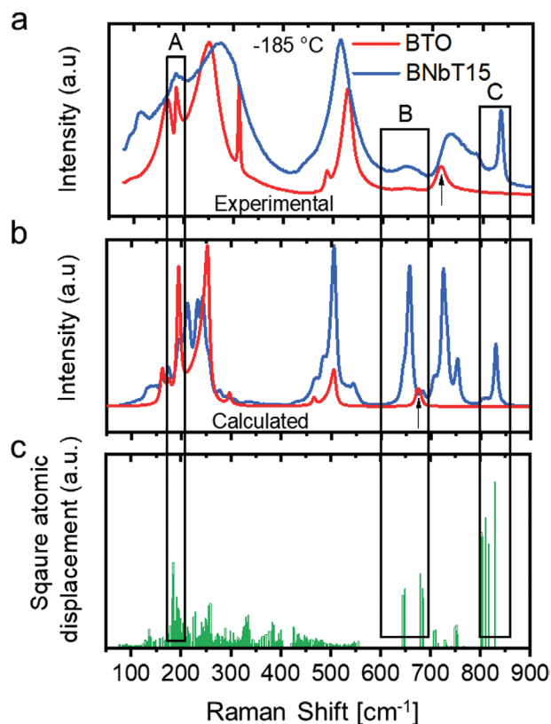
Figure 6. a) Measured Raman intensities for BTO and BNbT15 at -185^\circ\text{C} and b) the calculated Raman spectra of BTO and BNbT. c) Eigenmode analysis for six oxygen atoms around the titanium vacancy, where the sum of the square displacement of the six oxygen atoms is plotted for each mode. This analysis clearly describes the increased contribution of oxygen atoms to Raman-active phonons near the defect related modes that are marked as B and C.
